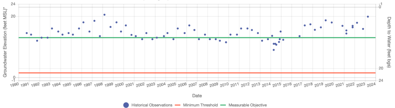
Hydrograph for Well: 02S07E31N001M
