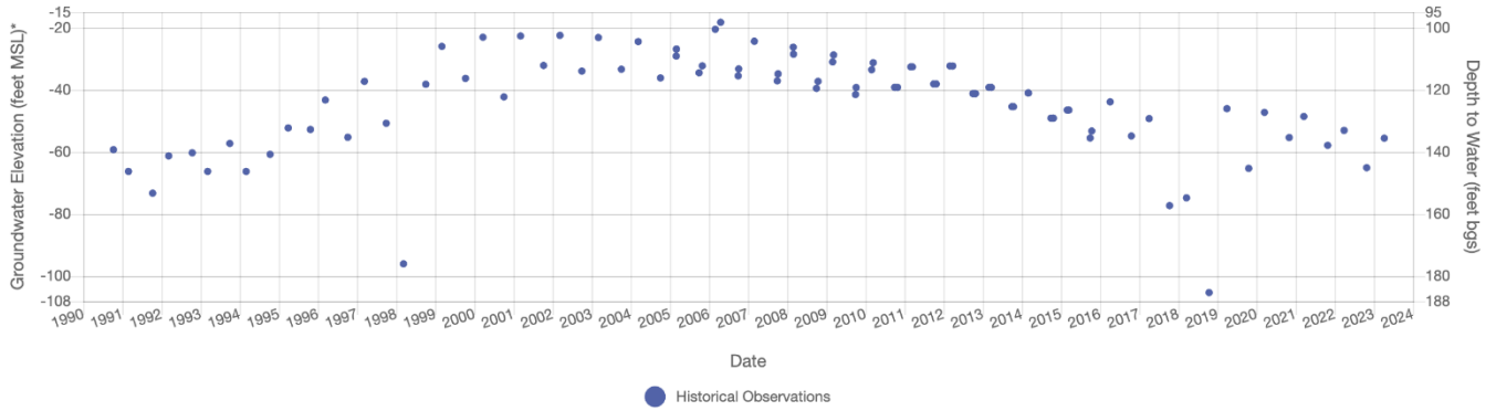
Hydrograph for Well: 01N08E16H002M
