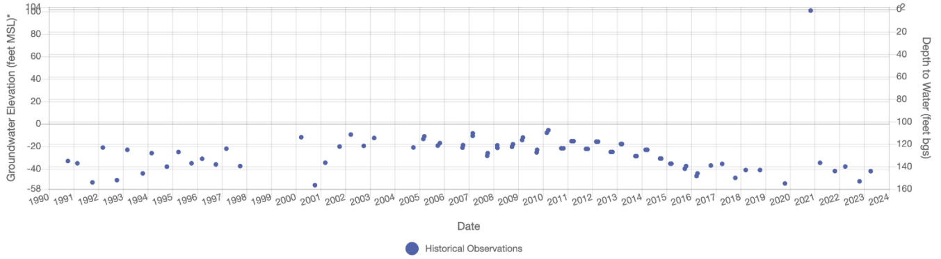
Hydrograph for Well: 01N09E17M001M
