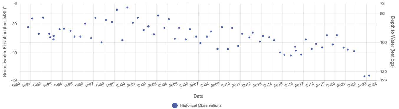
Hydrograph for Well: 04N07E17N001M
