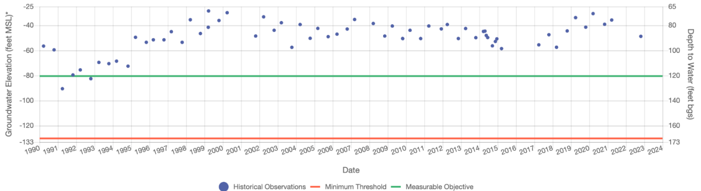
Hydrograph for Well: 02N07E29B001M
